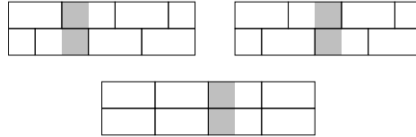
Fig. 6. Interference of coordinates for odd and even periods.
