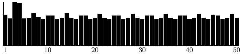
Fig. 5. Standard deviation test for a cryptogram of period 7
