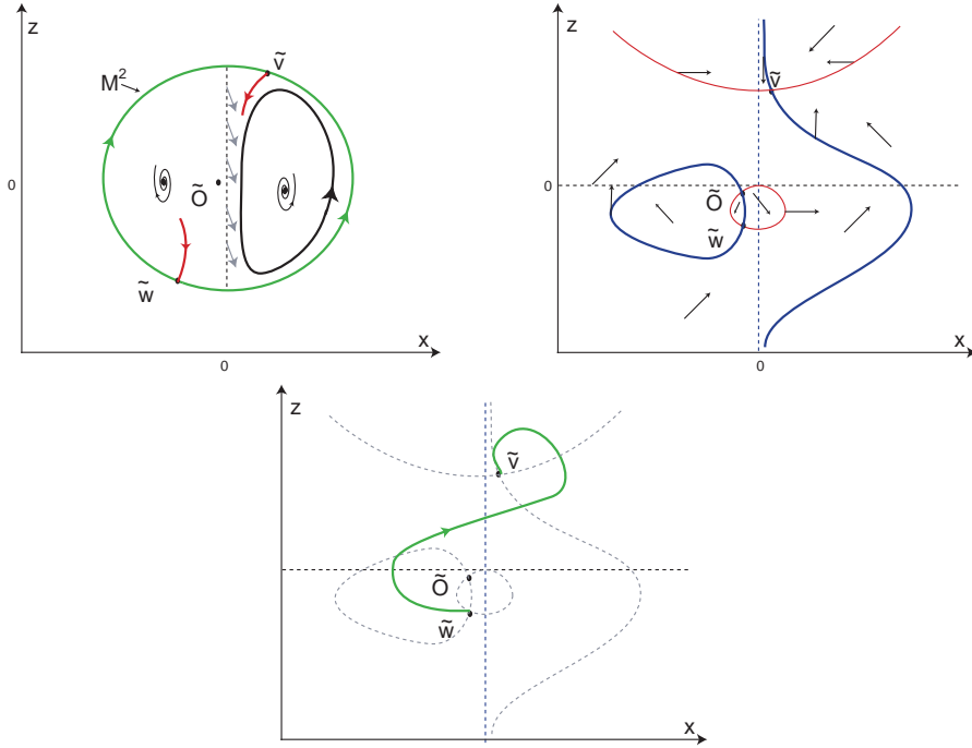
FIGURE 8. Qualitative phase portrait for the dynamics or (3.4) in \mathcal{M}^2 with y > 0 , projected into the (x_1, 0, x_3) plane for \mu = 0 and \nu > 0 .
