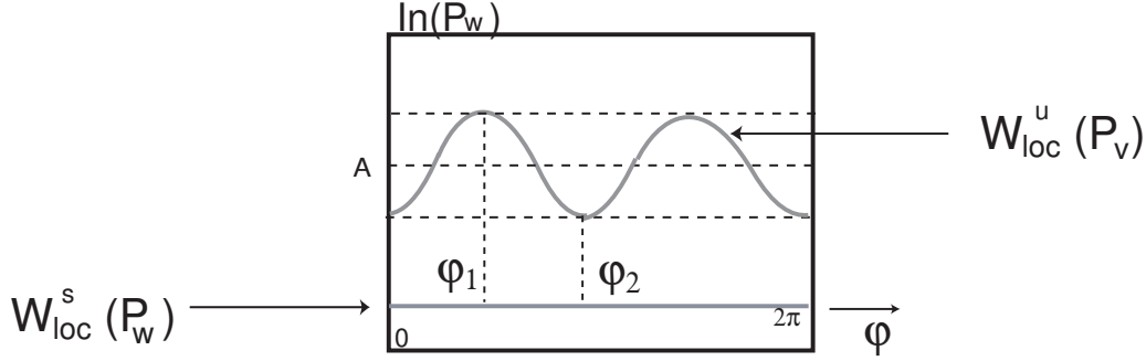
FIGURE 3. The local unstable manifold of \mathcal{P}_v intersects the cylinder In(\mathcal{P}_w) on a closed curve, the graph of a periodic Morse function \xi_{(\nu,\mu)} : \mathbf{R} \rightarrow [0, \varepsilon_w] with \nu > 0 , \mu > 0 .
