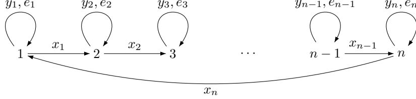
FIGURE 1. Underlying graph for the category C_n
