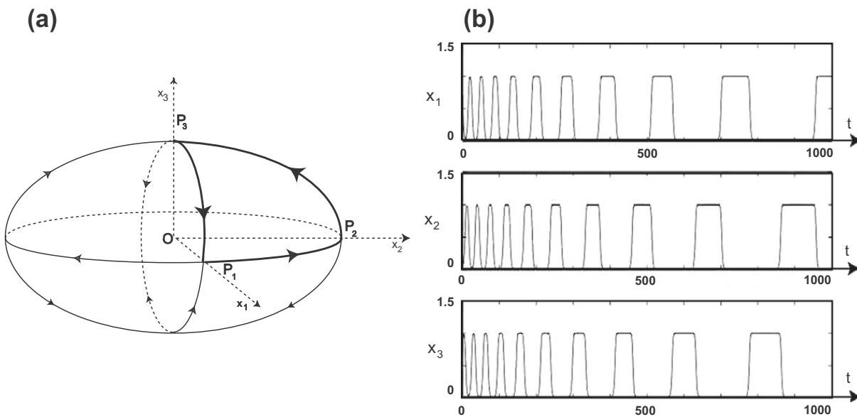
Fig. 5. (a) The network \Sigma_2 can be seen as the union of eight heteroclinic cycles (related by symmetry), each one lying on the boundary of each octant. The network \Sigma_2 is the \Theta -orbit of the cycle depicted on the first octant. (b) Time series for a trajectory starting in the first octant – it starts near the heteroclinic cycle approaching closer and closer the heteroclinic cycle, remaining near consecutive equilibria for increasing periods of time.
