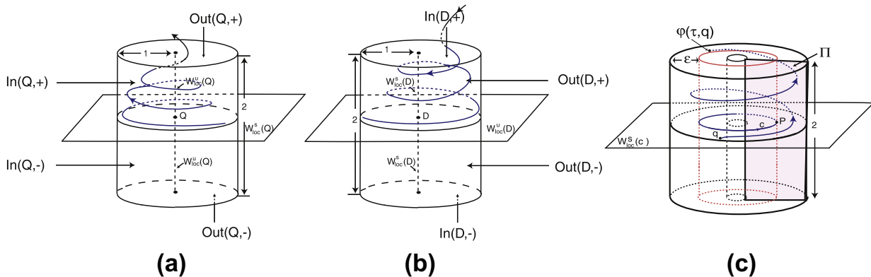
Fig. 7. (a) and (b) cylindrical neighbourhoods of the saddle-foci Q, D ; (c): hollow cylindrical neighbourhood of the non-trivial closed trajectory c .
