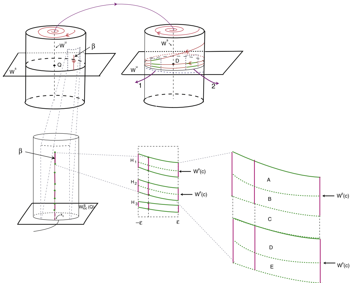
Fig. 9. On a segment \beta \subset In(Q) , there are infinitely many segments of initial conditions that follow the connections 1 and 2. There are infinitely many points that go away from the network. Varying x \in [-\epsilon, \epsilon] ( \epsilon > 0 small), each segment gives rise to a horizontal rectangle across In(Q) . Caption: A – points that follow the connection 1 and the upper part of C ; B – points that follow the connection 1 and the lower part of C ; C – points that go away from the network; D – points that follow the connection 2 and the upper part of C ; E – points that follow the connection 2 and the lower part of C .
