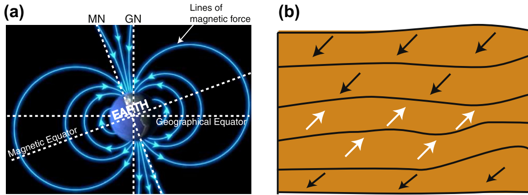
Fig. 1. (a) Scheme of the Earth's magnetic field, approximated as a magnetic axial dipole. Note that the locus of points with the same intensity of magnetic field is a closed curve; MN – Magnetic North; GN – Geographical North; (b) Scheme of the lava flow layers; the magnetic alignment preserved after cooling records reversion of the geomagnetic field. Each layer maintains the original magnetic field at its time of cooling.
