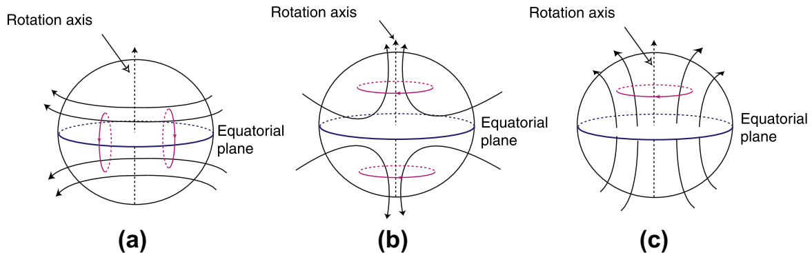
Fig. 3. Symmetric Modes. (a) Equatorial Dipole D_e ; (b) Axial Quadrupole Q_a ; (c) Axial Dipole D_a .
