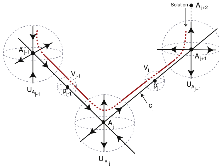
Fig. 2. Solution shadowing a path of order 3, in a three-dimensional manifold: given the three heteroclinic connections [A_{j-1} \rightarrow A_j] , [A_j \rightarrow A_{j+1}] and [A_{j+1} \rightarrow A_{j+2}] , there is a solution following them.
