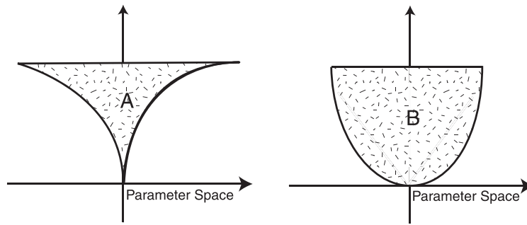
Fig. 4. The set A is not a large set (bounded by tangent lines) and B is a large set. The origin represents the bifurcation point.
