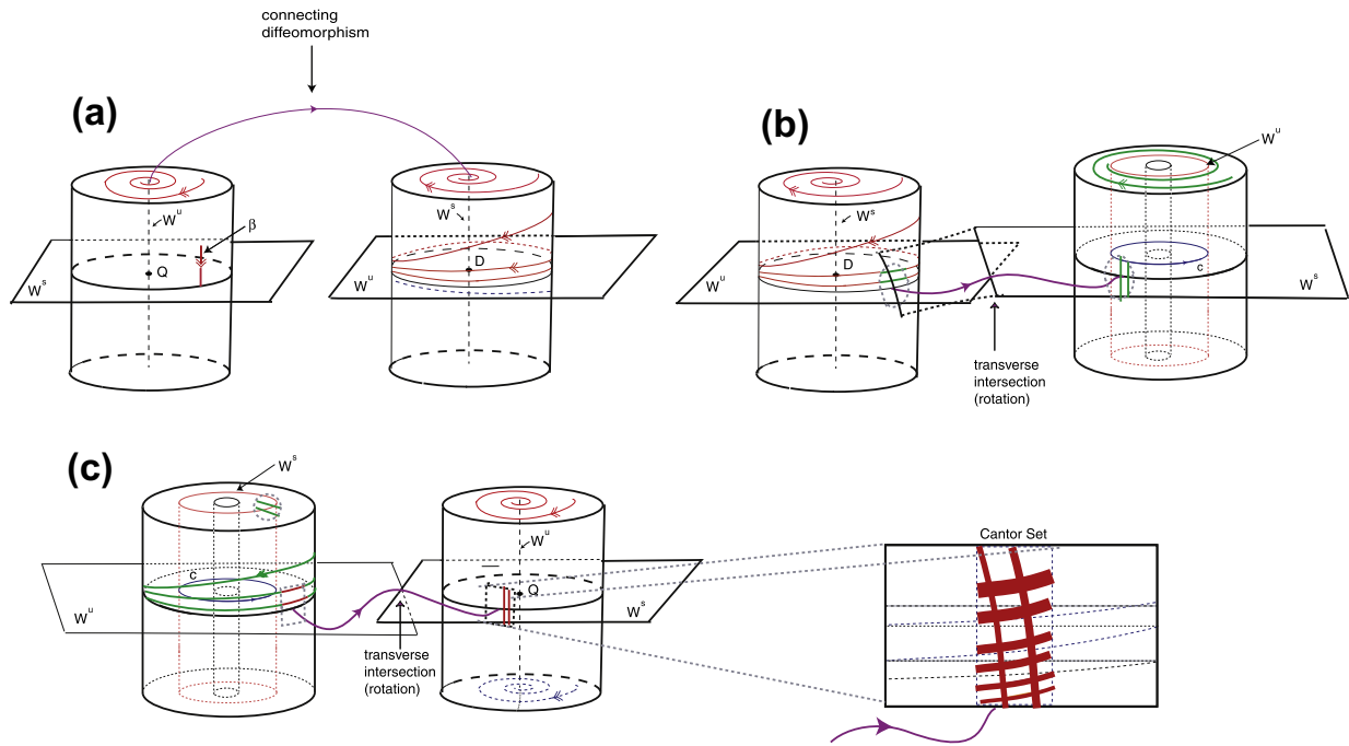
Fig. 8. Local and global dynamics near the heteroclinic network. (a) A segment of initial conditions lying across the stable manifold of Q is mapped, by the local map \phi_1 , into a spiral accumulating on its unstable manifold and thus on the stable manifold of D ; (b) a spiral of initial conditions on the top of the neighbourhood of D is mapped, by the local map \phi_2 , into a helix accumulating on the unstable manifold of D , which crosses transversely the stable manifold of c infinitely many times; (c) a segment of initial conditions lying across the stable manifold of c is mapped into a spiral accumulating on its unstable manifold. Each piece of helix is a new segment across the stable manifold of Q . In (c), it is also possible to observe the first step of the construction of the Cantor set on the wall of the cylinder ln(Q) .
