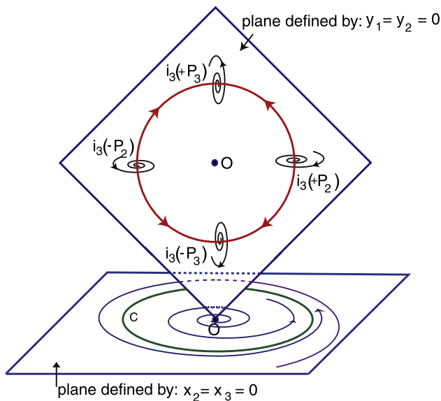
Fig. 6. Representation of the two planes Fix(\mathbf{SO}(2)) (horizontal) and Fix(\mathbf{Z}_2 \oplus \mathbf{Z}_2) (vertical), in which the invariant saddles associated to \Sigma_3 lie. In Fix(\mathbf{SO}(2)) , the non trivial closed trajectory c is a sink; in Fix(\mathbf{Z}_2 \oplus \mathbf{Z}_2) , we observe the non robust heteroclinic connections of the network which do not involve c . Note that \mathbf{R}^4 = Fix(\mathbf{SO}(2)) \oplus Fix(\mathbf{Z}_2 \oplus \mathbf{Z}_2) .
