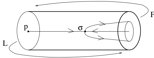
FIGURE 3. A sketch of the construction of a singular-attractor in higher dimensions
