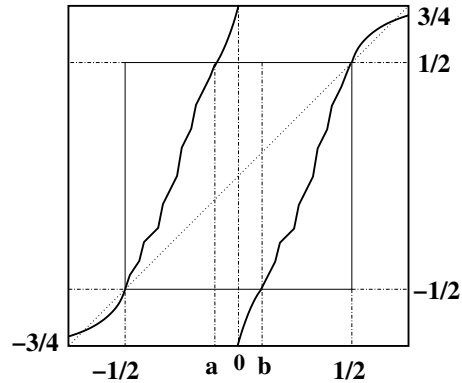
FIGURE 1. The one-dimensional Lorenz-like map.
