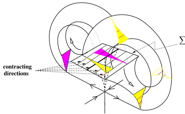
FIGURE 2. The geometric Lorenz attractor with the contracting directions on the cross-section \Sigma .
